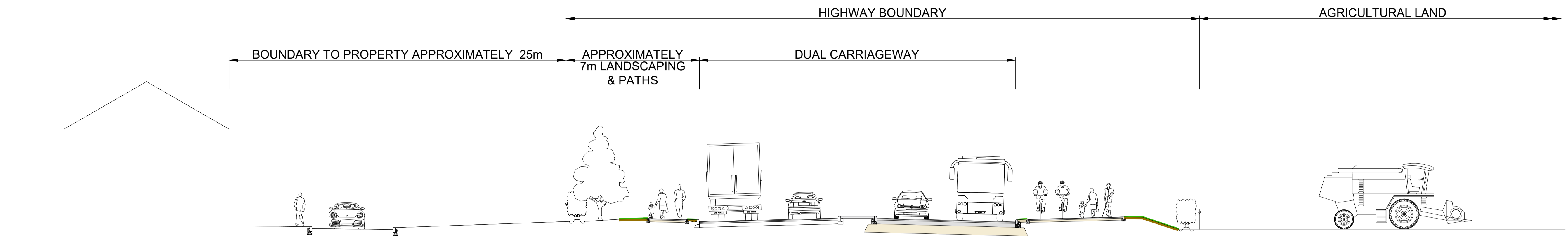
Typical Cross Section - Portland Wynd Area
