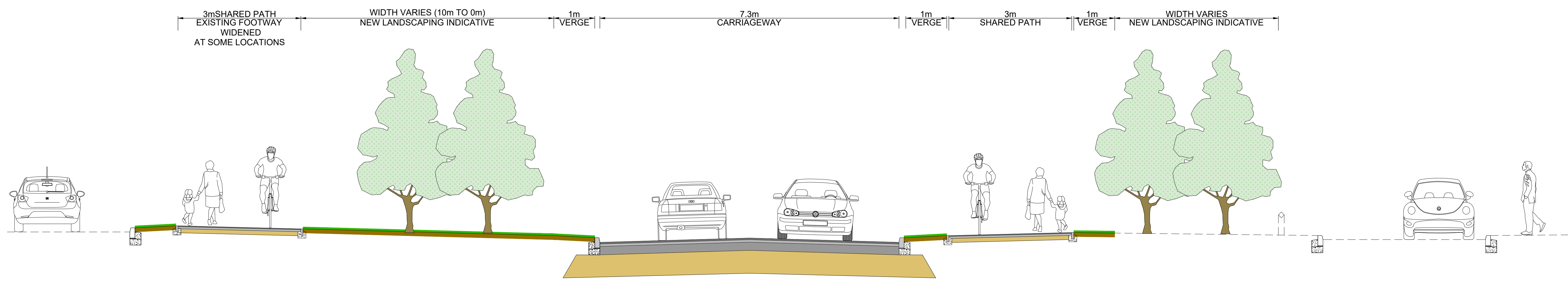
Typical Cross Section - West of Tynedale Drive
